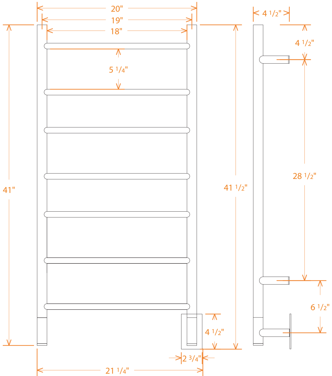
FRONT VIEW OF RACK ON WALL
