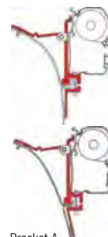
Bracket A
