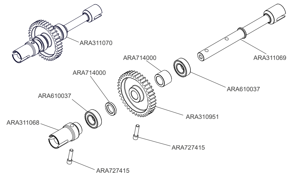
CENTER SPOOL EXPLODED VIEW
