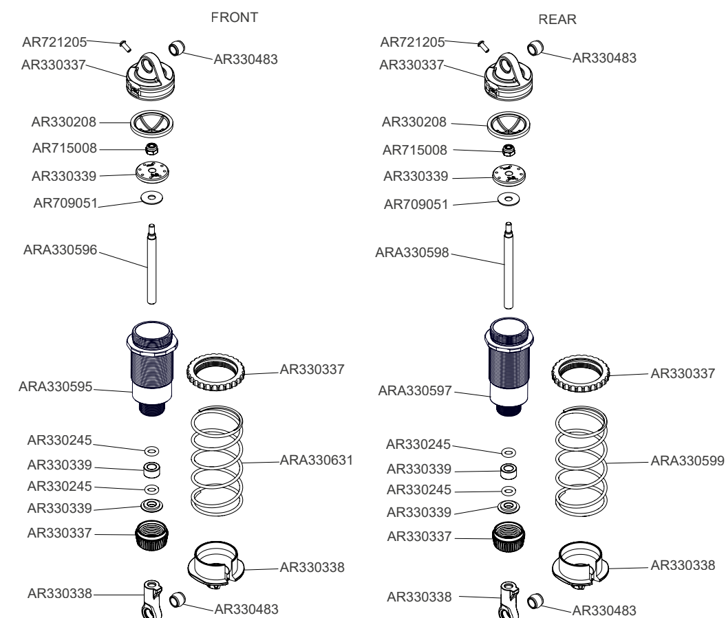
SHOCK ABSORBER EXPLODED VIEW
