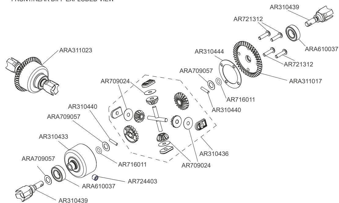
FRONT/REAR DIFF EXPLODED VIEW
